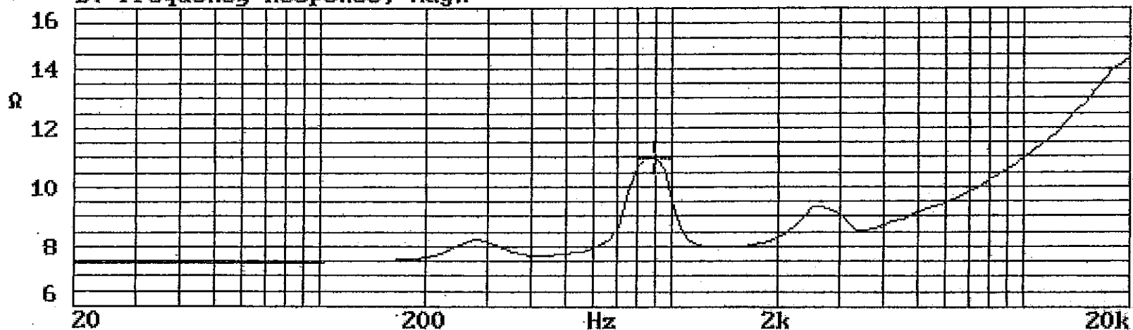
B: Frequency Response, Magn
